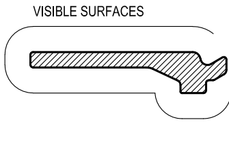
UCW158 136mm SSG 28-30mm IGU GLAZING SEAT Mass. 0.398 Kg/m Anod. Per. 89 Paint Per. 100
