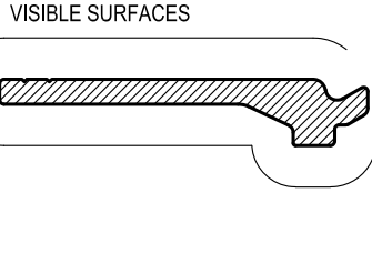
UCW160 136mm SSG 36-38mm IGU GLAZING SEAT Mass. 0.446 Kg/m Anod. Per. 101 Paint Per. 100
