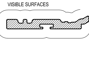
UCW165 136mm SSG 32-34mm IGU GLAZING BEAD Mass. 0.463 Kg/m Anod. Per. 115 Paint Per. 100
