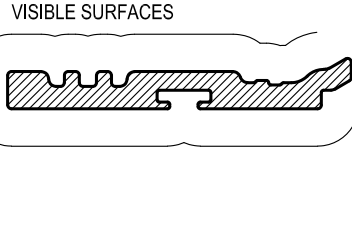
UCW166 136mm SSG 36-38mm IGU GLAZING BEAD Mass. 0.491 Kg/m Anod. Per. 123 Paint Per. 100
