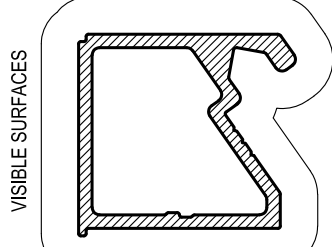
UCW163 136mm SSG SINGLE GLAZE ADAPTOR 26mm Mass. 0.560 Kg/m Anod. Per. 124 Paint Per. 100
