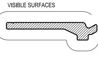
UCW159 136mm SSG 32-34mm IGU GLAZING SEAT Mass. 0.422 Kg/m Anod. Per. 95 Paint Per. 100
