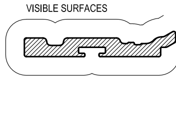
UCW164 136mm SSG 28-30mm IGU GLAZING BEAD Mass. 0.428 Kg/m Anod. Per. 106 Paint Per. 100
