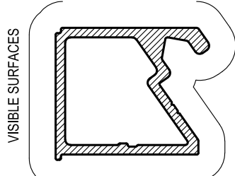
UCW162 136mm SSG SINGLE GLAZE ADAPTOR 24mm Mass. 0.540 Kg/m Anod. Per. 120 Paint Per. 100
